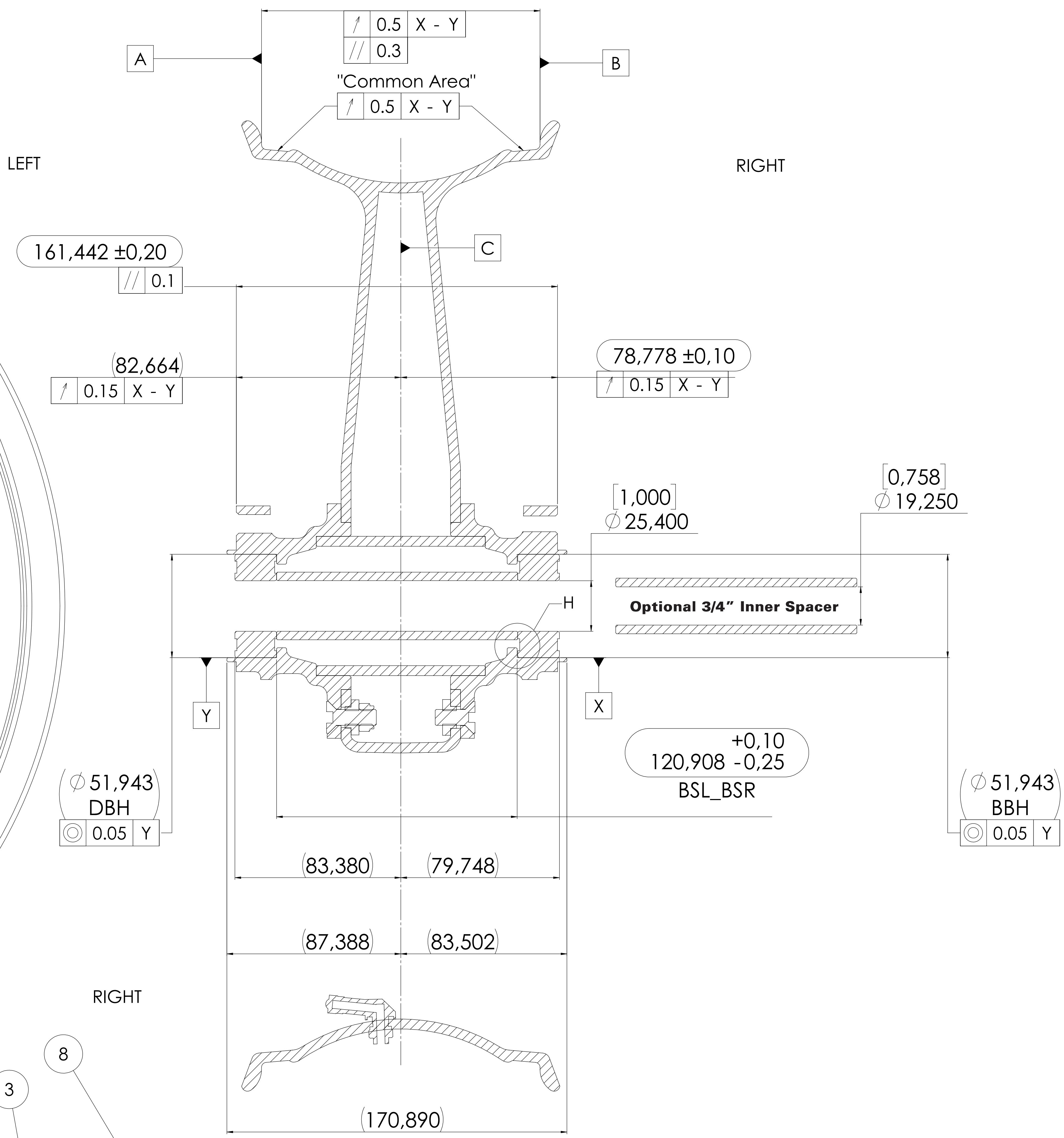
SECTION G-G
