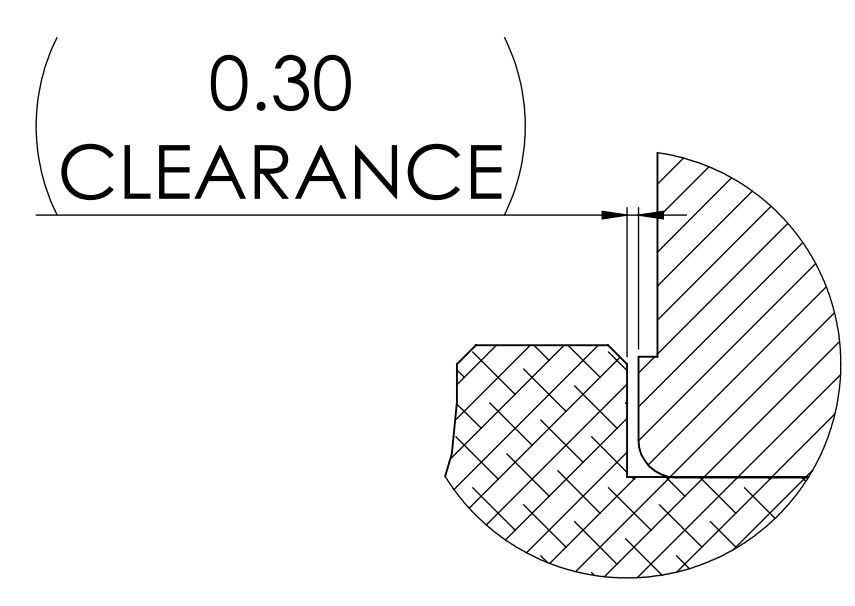
DETAIL B SCALE 5 : 1
