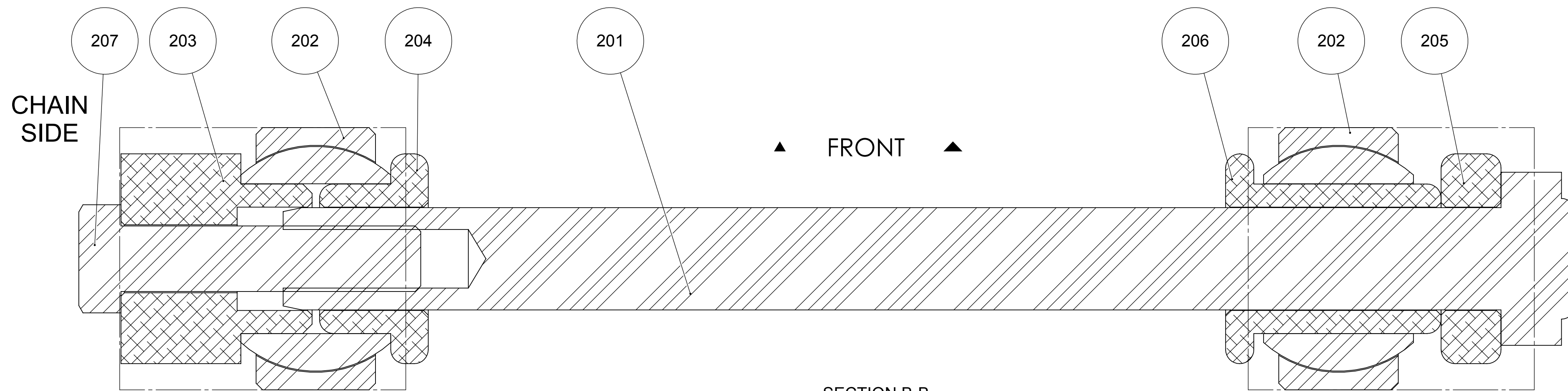
SECTION B-B
