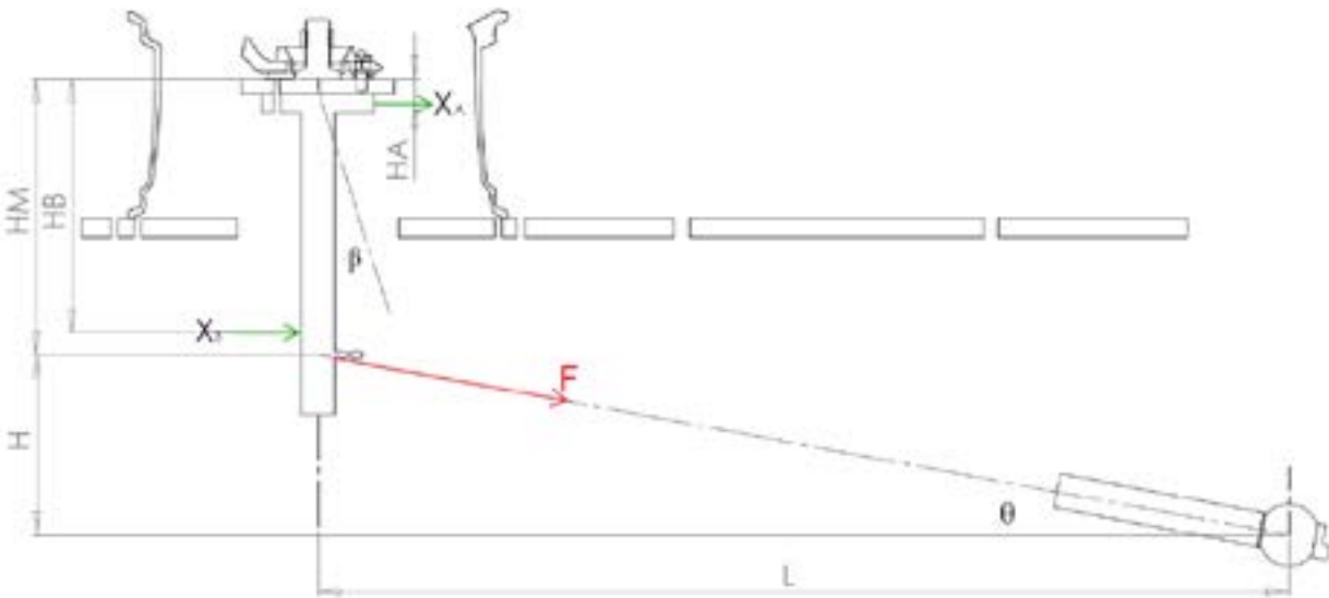
Fig. 03 Bending Stiffness Experiment
