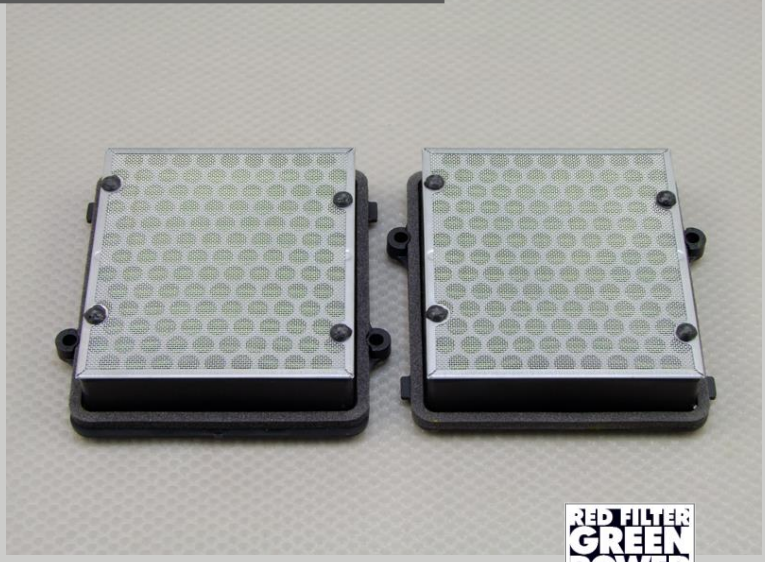
P-H10E16-01 vs 17210-MJP-G50 / Bottom side
